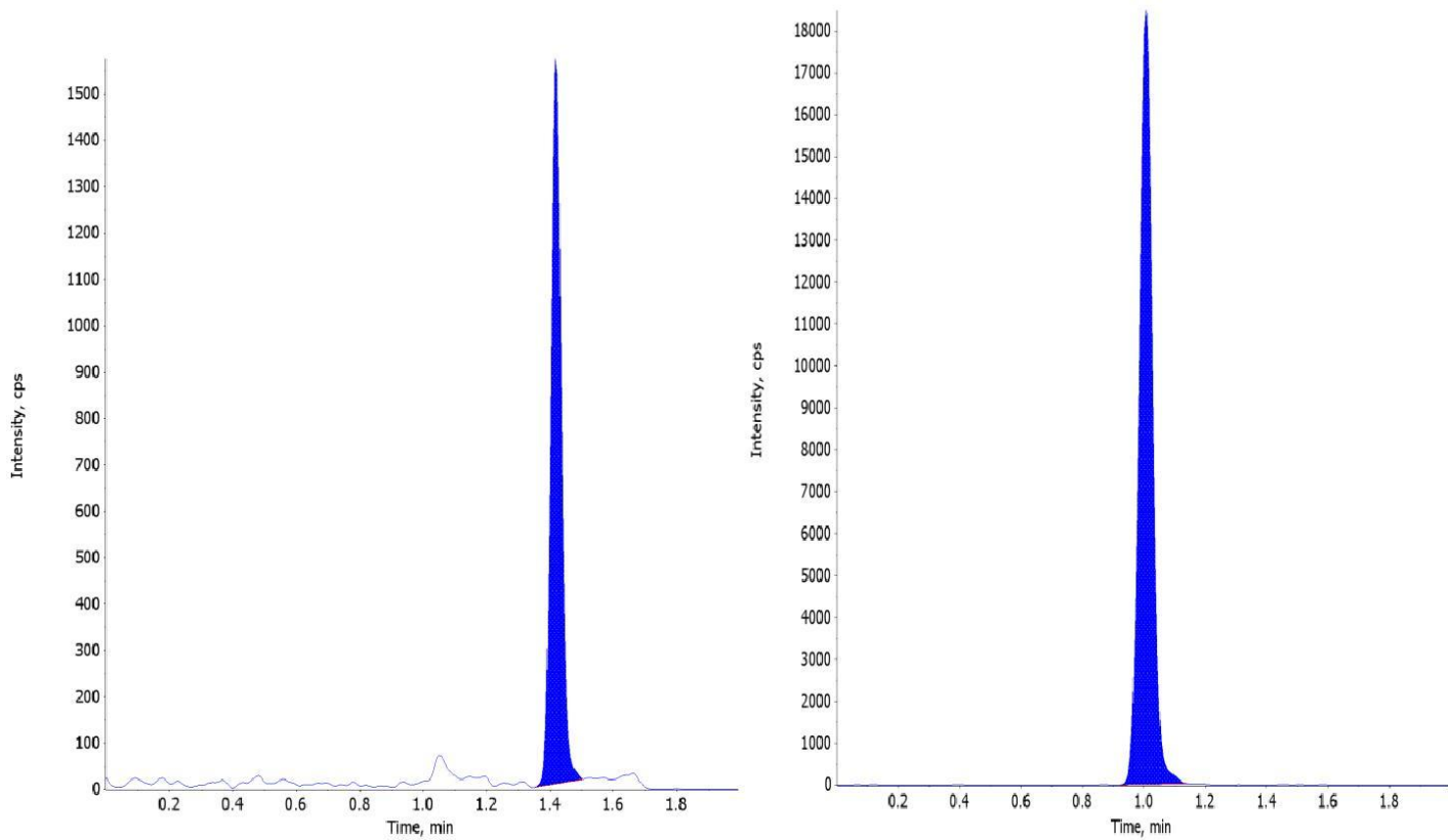
Figure 42: Candesartan LLOQ chromatogram.
